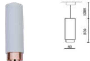
Fitting-Suspended-GU10
