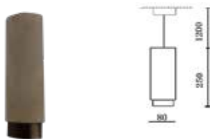
Fitting-Pendant Metal-1XGU10
