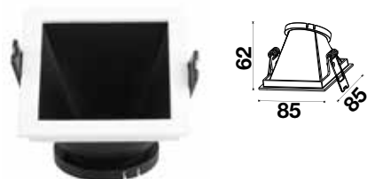
Fitting Square-GU10
