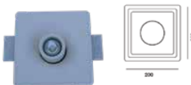
Fitting-Ceiling Metal-1XGU10
