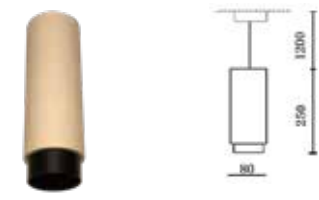
Fitting-Pendant Metal-1XGU10
