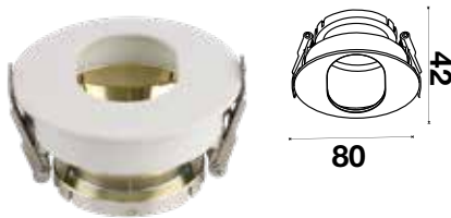
Fitting Round-GU10
