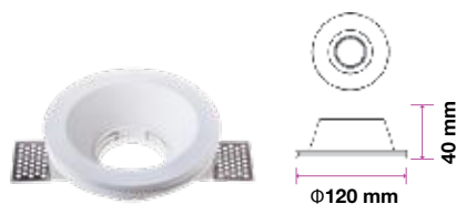
Fitting-Round-GU10
