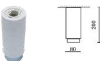
Fitting-Surface Metal-1XGU10
