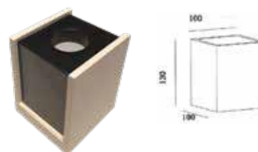
Fitting-Square Metal-1XGU10
